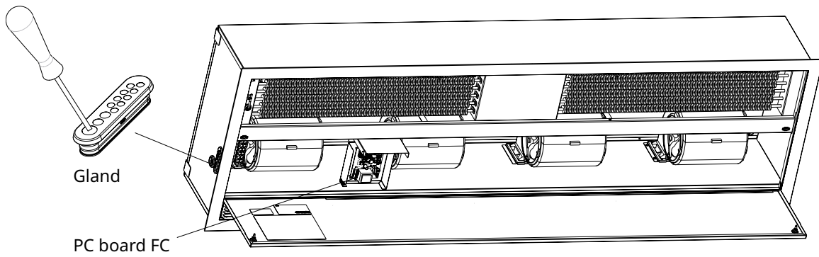
Fig. 4: PC board FC is integrated within the air curtain at delivery.
