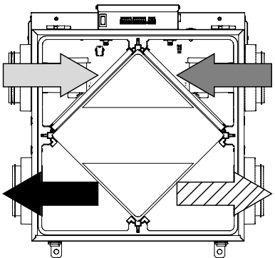
Standard ERV Airflow
